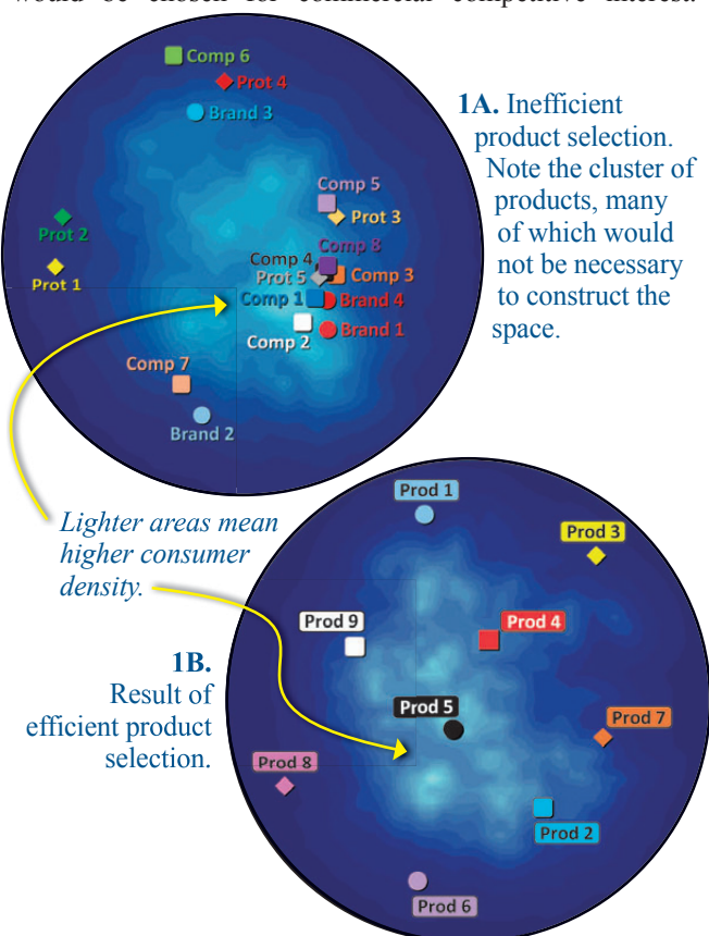
Figure 1A-B. Landscape Segmentation Analysis® (LSA) maps of products and ideal point densities resulting from selecting inefficient (A) and efficient (B) products.
